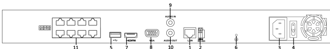
Figure 2 DS-7608NI-SE/P Rear Panel
